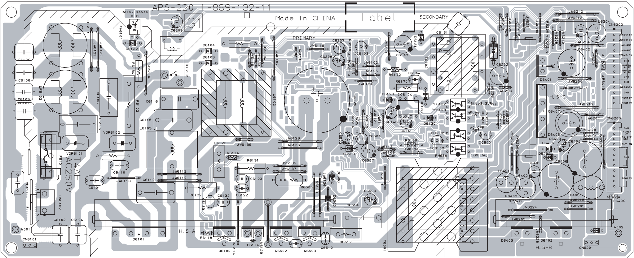
<COMPONENT SIDE>
