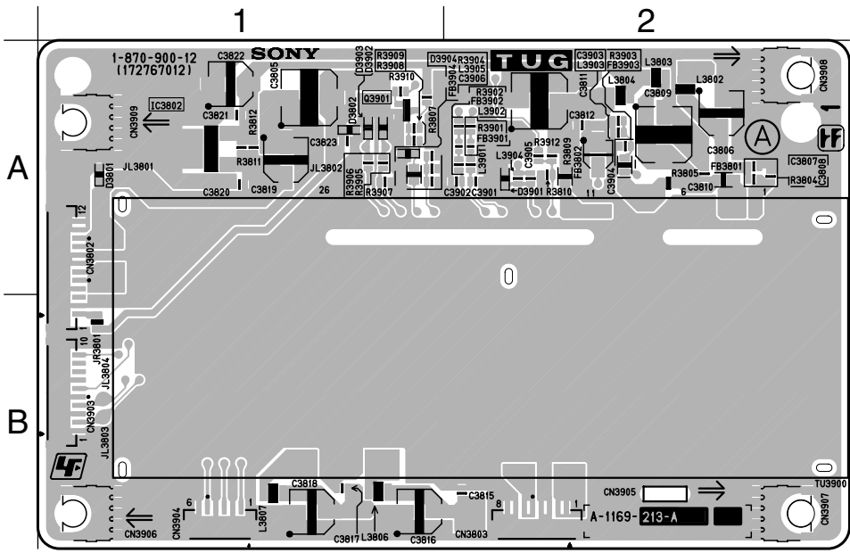
<COMPONENT SIDE>
